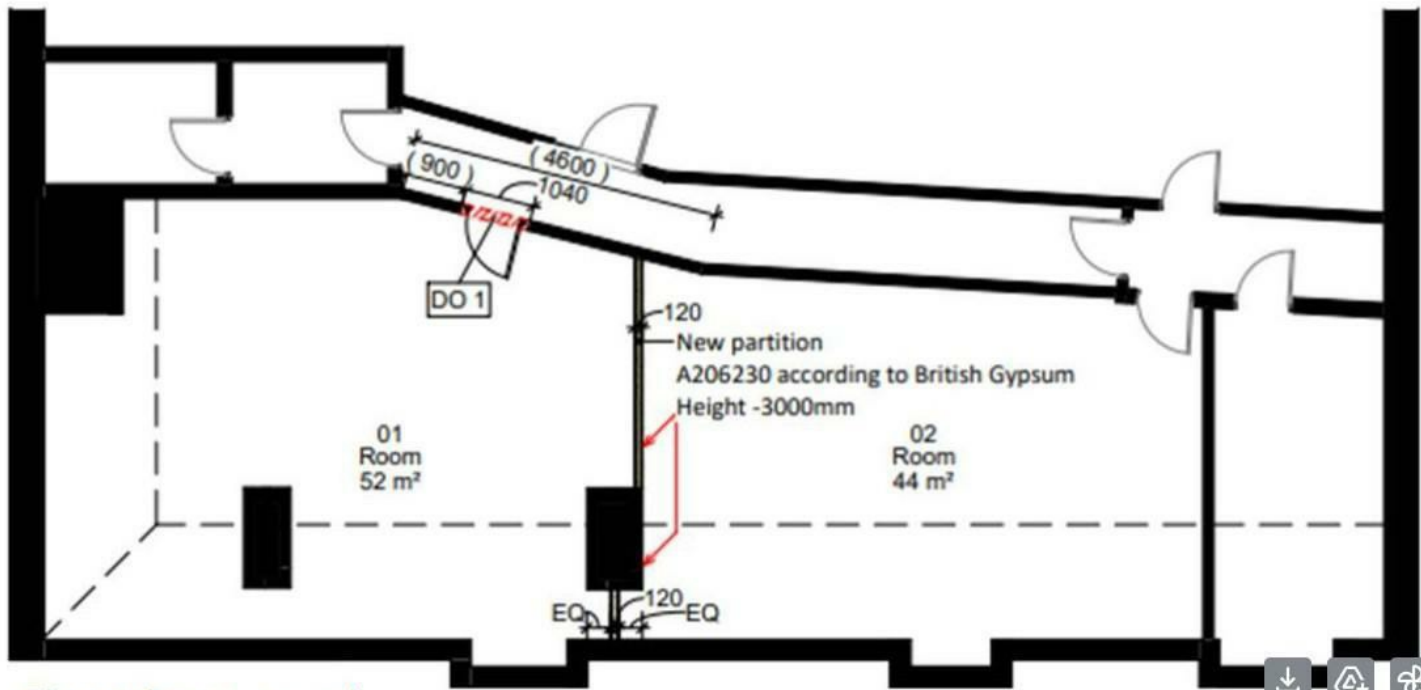
Floor plan proposal
